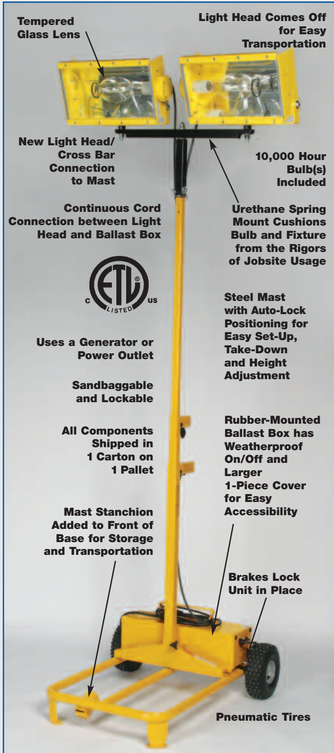
Rolls Anywhere—fits through a 32" door!
